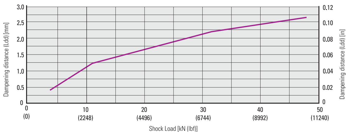
Dampening Distance vs. Shock Load
