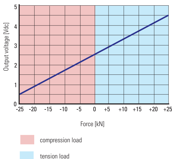
Force vs. Force Feedback Output Voltage
