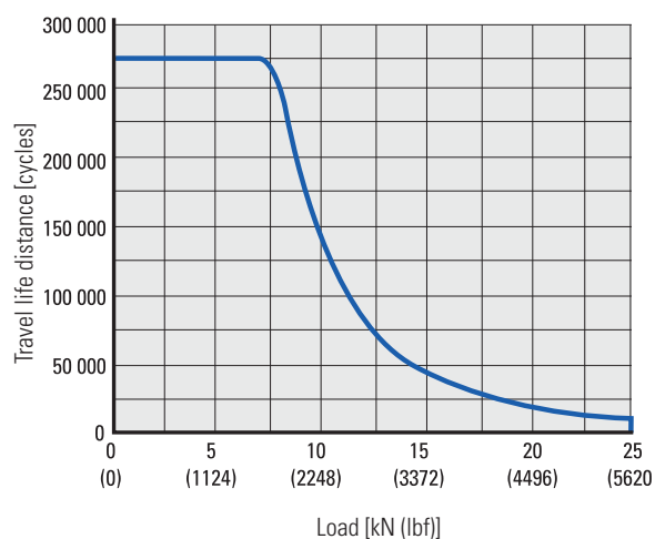
Estimated Life vs. Load
