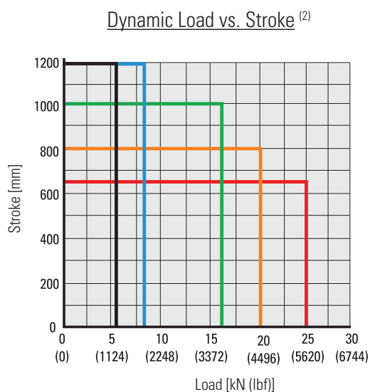
Actuator Dynamic Load Capacity Rating
