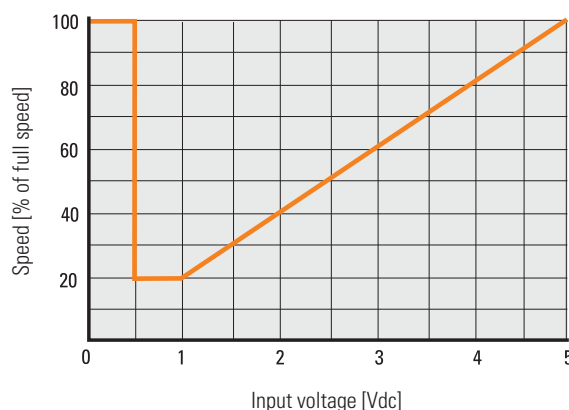
Speed vs. Speed Control Input Voltage
