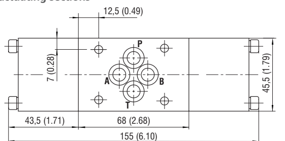
Valve with three positions two actuating sections
