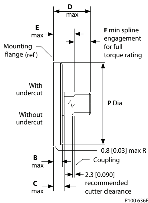
Auxiliary pump mating dimensions mm [in.]
