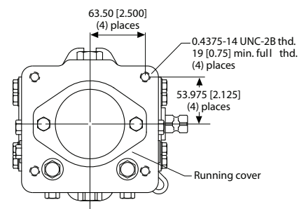
Running cover
