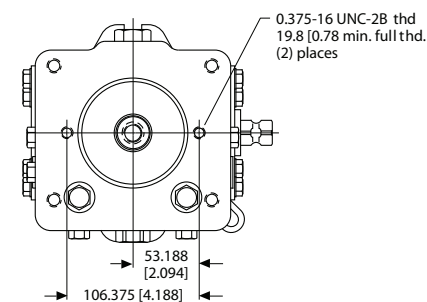
SAE A Auxiliary mounting flange
