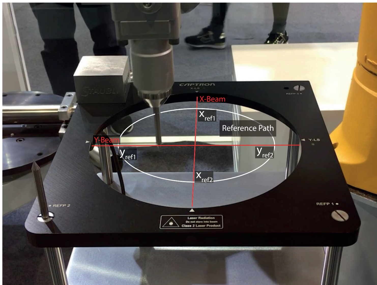
Figure 2: TCP reference measurement
