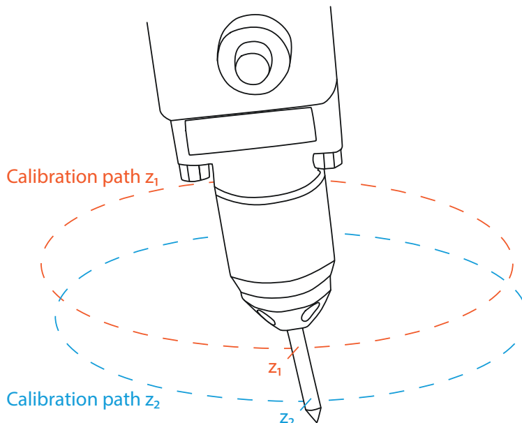
Figure 3: Tilt correction calibration path
