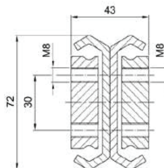
NTV72-43DC
