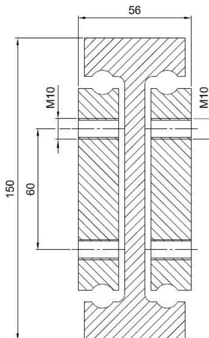
NTS150-56
