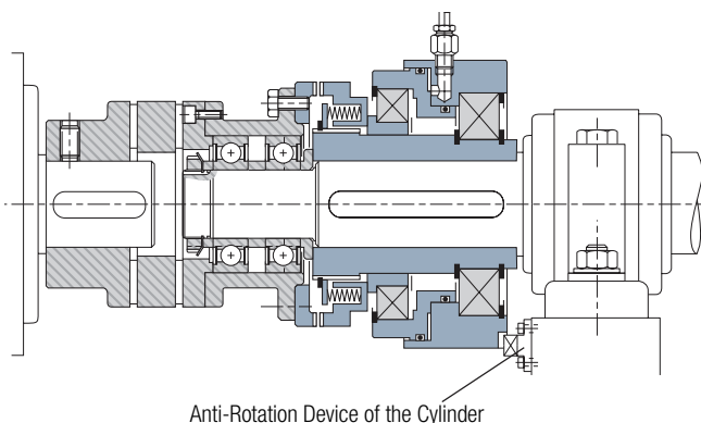
Mounting Example
