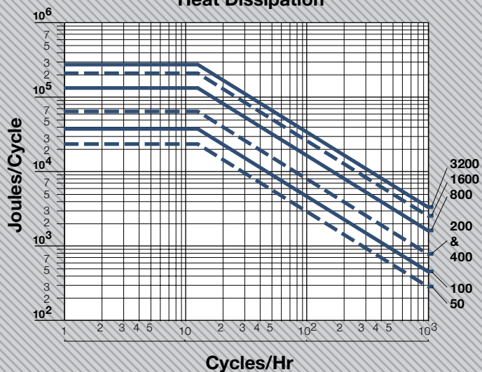
Heat Dissipation
