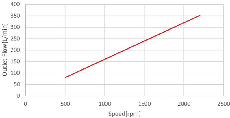
193cc flow vs speed
