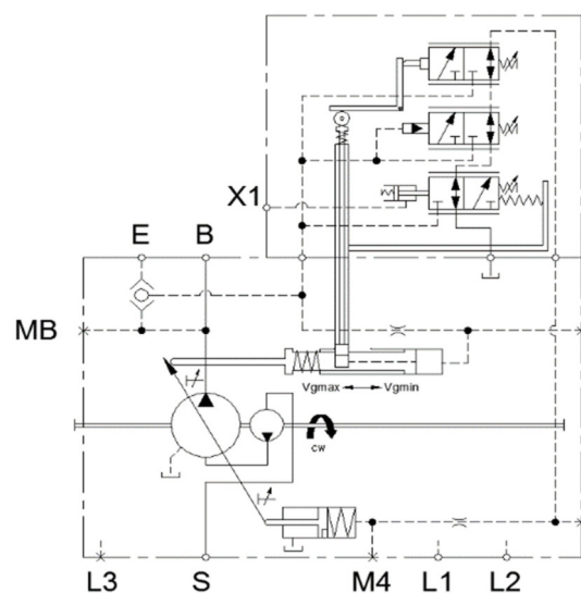
Schematic
