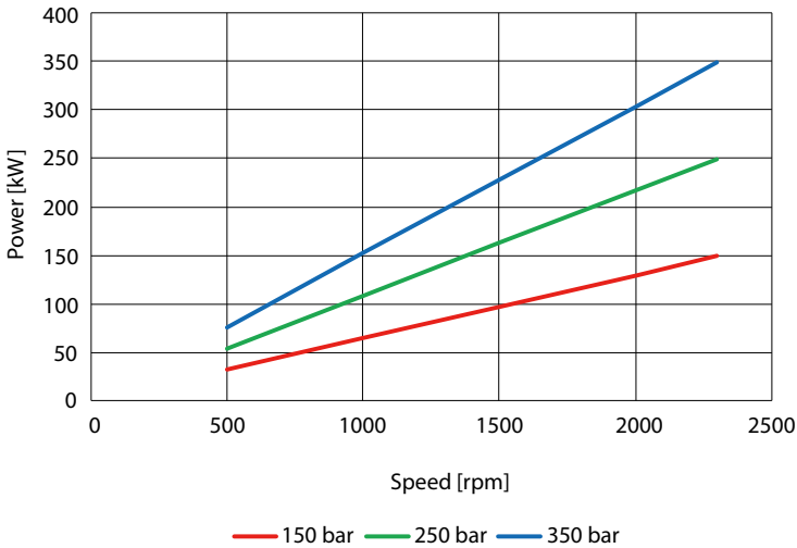
260cc power vs input speed
