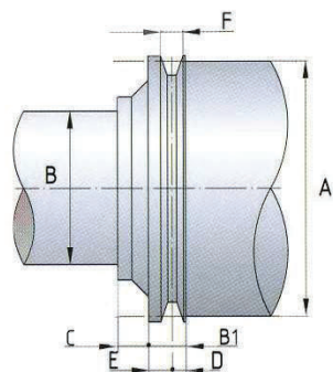
Trapezoidale / Sheave for V belt Keilriemenscheibe / Trapezoidale
