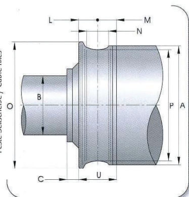
Fissa funi / Fixed sheave for rope Feste Seilscheibe / Cable fixes
