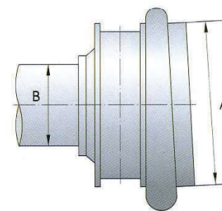
Orientabile / Swinging head Schwenkbare Scheibe / Orientable
