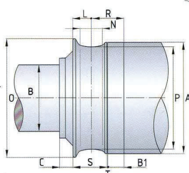
Folle funi / Idle sheave for rope Lose Seilscheibe / Cable fous
