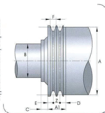
2 trapezoidal / Double sheave for V belt Doppelkeilriemenscheibe / 2 trapezoidale
