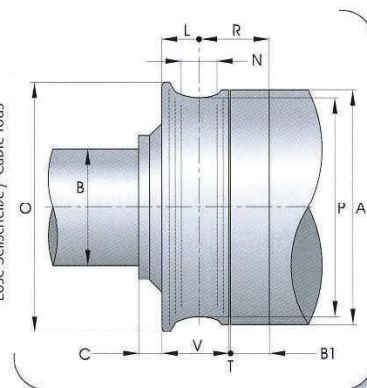
Folle funi / Idle sheave for rope Lose Seilscheibe / Cable fous
