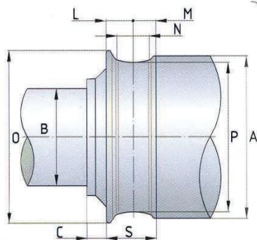
Fissa funi / Fixed sheave for rope Feste Seilscheibe / Cable fixes
