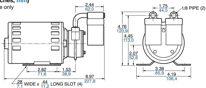
Model 1531 (AC Motor)
