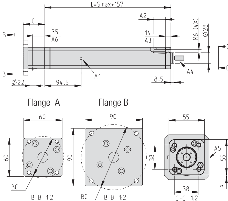
Dimensions for Inline Style with RediMount Motor Flange
