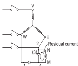
Fig. 1 Standard Circuit
