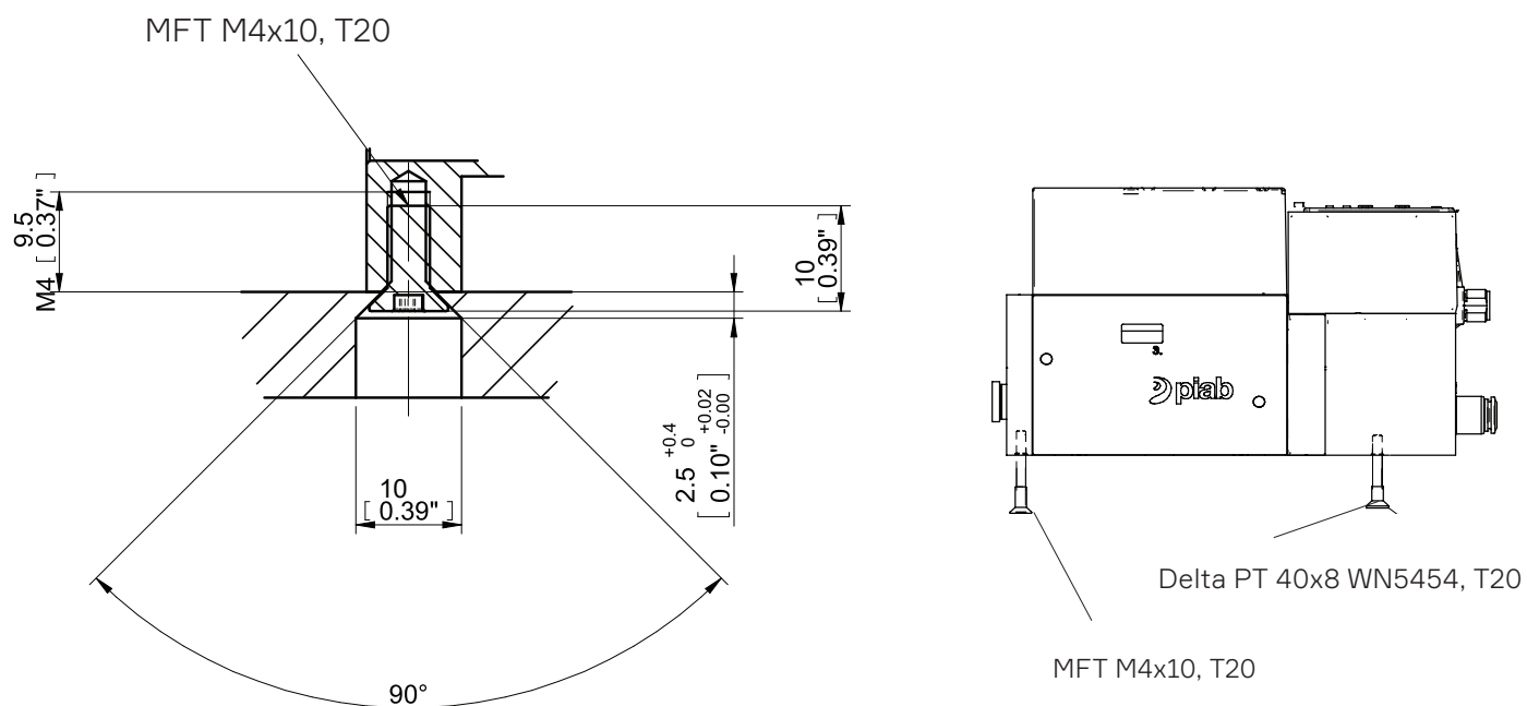
Figure 12 Bez filtra.
