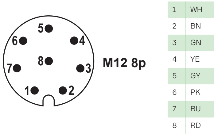
Figure 6 M12 8p
