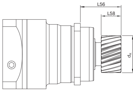
PSN/PLN with pinion (also applies to WPLN, PLHE and WPLHE)
