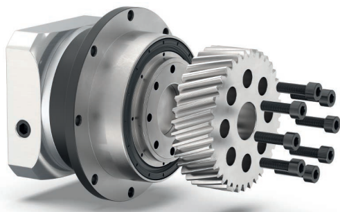
PSFN090 with PM1 pinion for gearbox frame size 090
