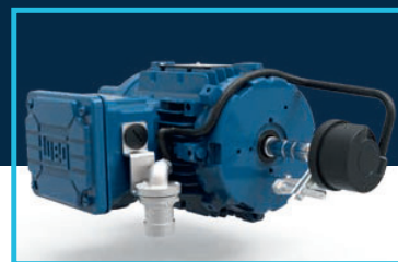
Incremental encoder (forced ventilation)
