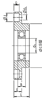
Hole pattern with 6 holes
