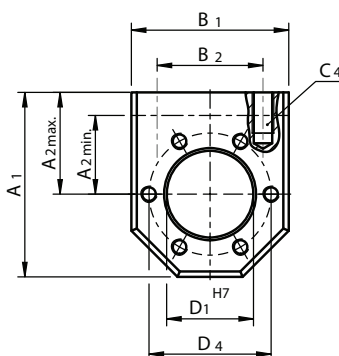
Hole pattern 3
