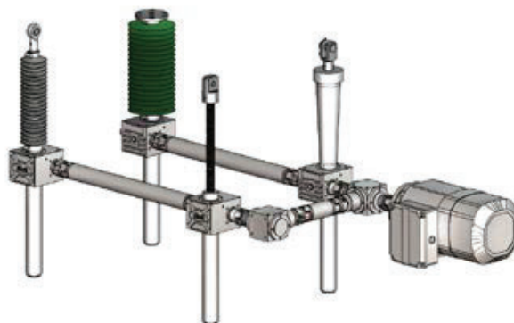
Four screw jacks in different configurations driven by a single motor
