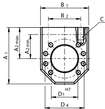
Hole pattern 2 according to DIN 69051
