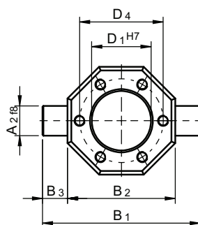
Hole pattern 3
