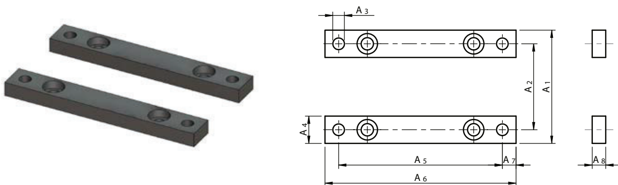
Dimensions [mm]
