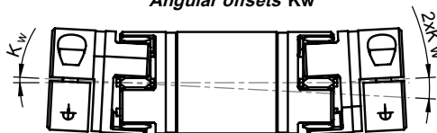
Angular offsets K_w
