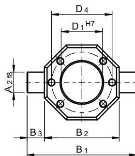
Hole pattern 3
