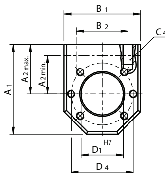
Hole pattern 1 according to DIN 69051
