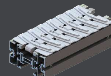
Single strand flexible chain - tab version
