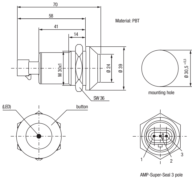
145...AB with Superseal connector
