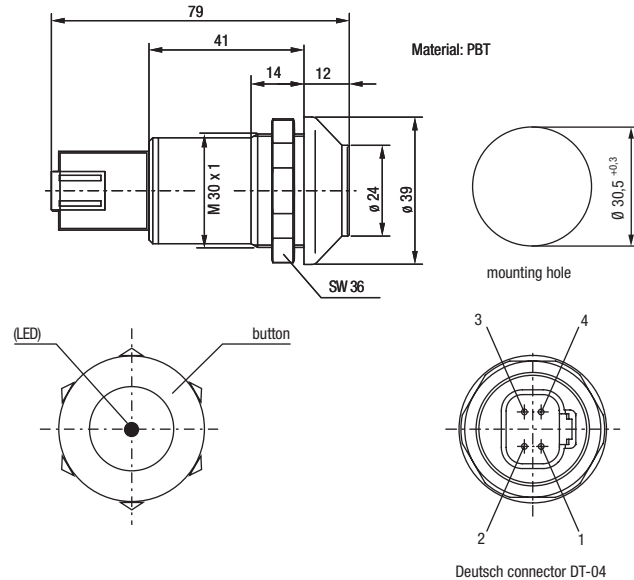
145...AE with Deutsch connector
