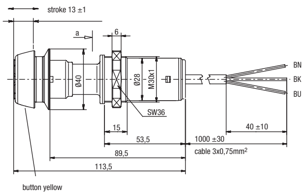
145PT010A00 power take-off switch with cable
