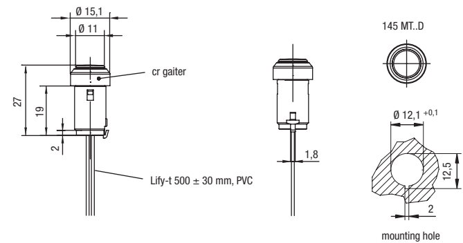
145MT..D with latching detent
