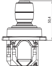
J1 with grip and integrated push button
