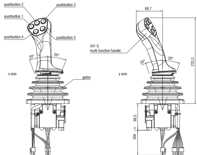
J4 joystick with joystick grip 341G...
