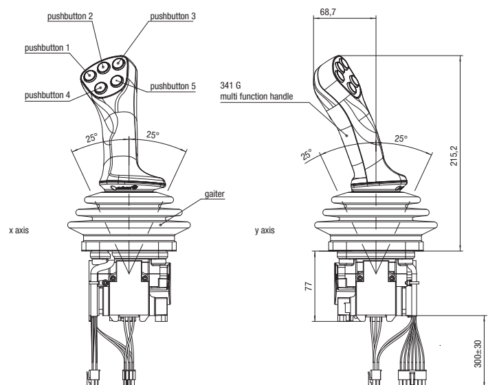
J5 joystick with joystick grip 341G...
