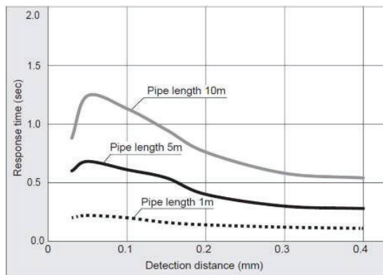
● Effect of pipe length on response time (OFF → ON)
