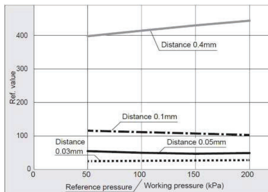
● Effect of working pressure change on reference value
