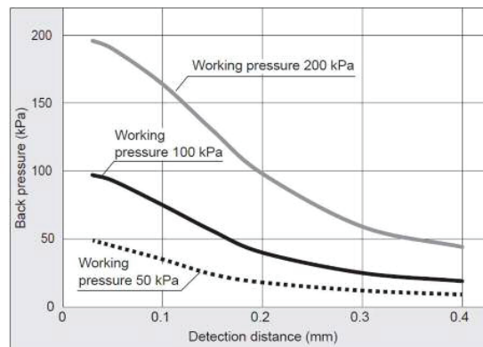
● Back pressure characteristic 2 - Differences in back pressure change due to working pressure
