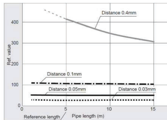
● Effect of pipe length change on reference value
