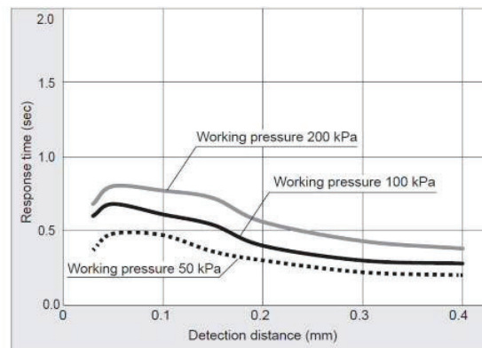
● Effect of working pressure on response time (OFF → ON)
