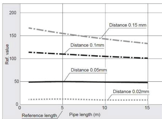
● Effect of pipe length change on reference value
