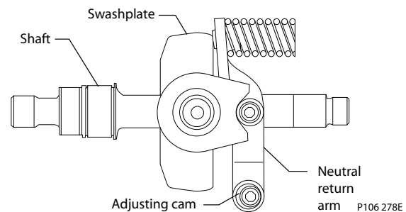
Neutral return mechanism
