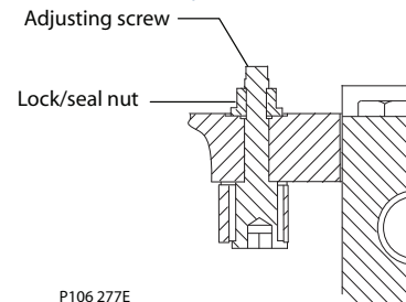
Neutral return mechanism
