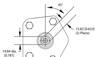
CONTROL TRUNNION DETAIL
