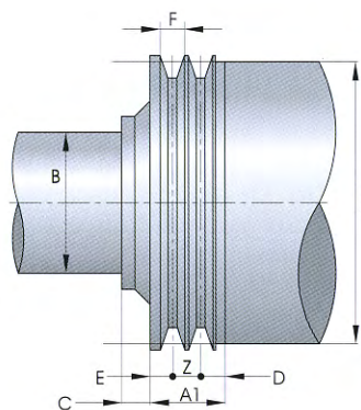
2 trapezoidali / Double sheave for V belt Doppelkellriemenscheibe / 2 trapezoidale
