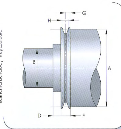
Trapezoidale / Sheave for V belt keilriemenscheibe / Trapézoidale
