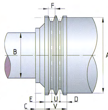
2 trapezoidali / Double sheave for V belt Doppelkeilriemenscheibe / 2 trapezoidale
