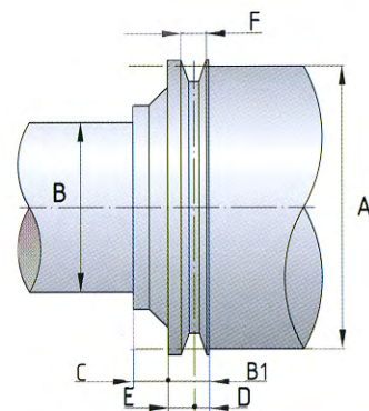
Trapezoidale / Sheave for V belt Keilriemenscheibe / Trapezoidale
