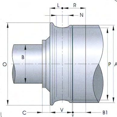
Folle funi / Idle sheave for rope Lose Seilscheibe / Cable fous
