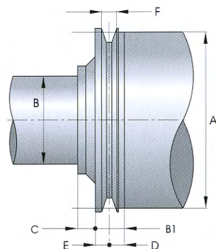
Trapezoidale / Sheave for V belt Kellriemenscheibe / Trapezoidale
