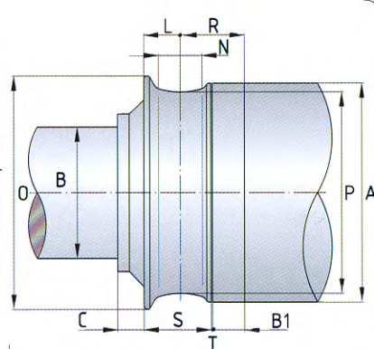
Folle funi / Idle sheave for rope Lose Seilscheibe / Cable fous
