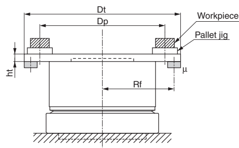
(Fig. 1) load conditions
