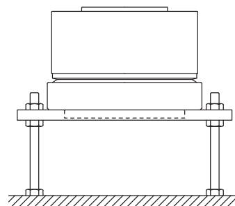
(Fig. 4) installation rigidity: low
