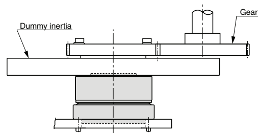
[Fig. 4] Example 2, dummy inertia installation
