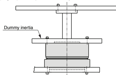
[Fig. 3] Example 1, dummy inertia installation
