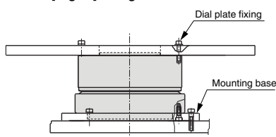
[Fig. 1] fixing of actuator
