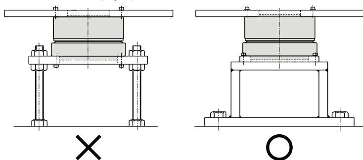
[Fig. 2] installation of actuator
