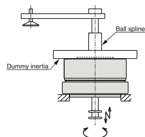
[Fig. 5] Example 3, dummy inertia installation
