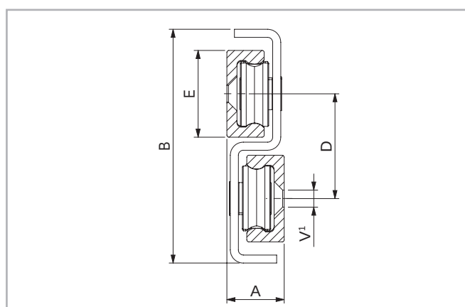
1 Fixing holes (V) for countersunk head screw according to DIN 7991
