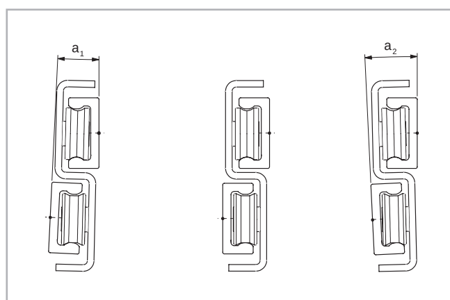
TLR..AP Self-aligning version available for all sizes (see pg. TL-27)
