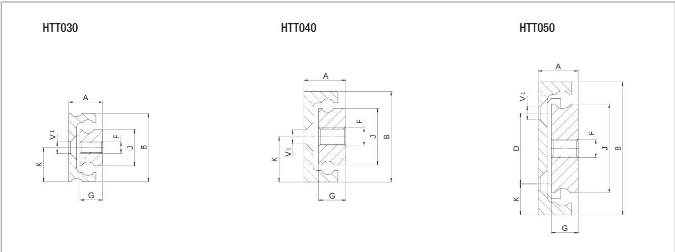
All dimensions are indicated in mm 1 Mounting holes (V) for countersunk screws according to DIN 7991/ISO 10642
