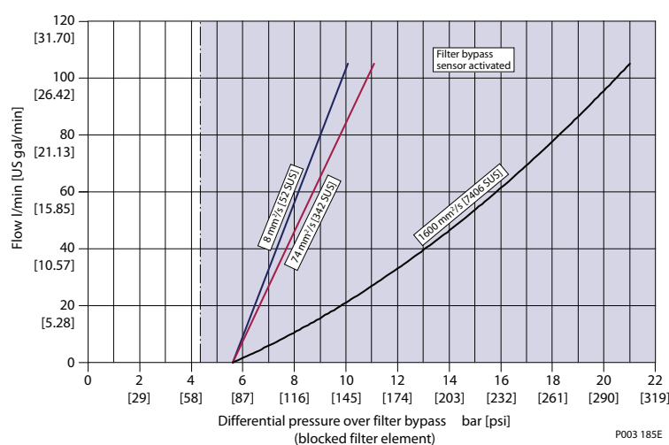
Filter bypass characteristic (completely blocked element)
