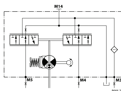
MDC schematic diagram
