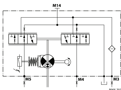
MDC NSS schematic diagram
