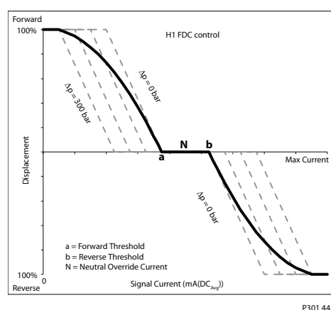
Pump displacement vs. control current
