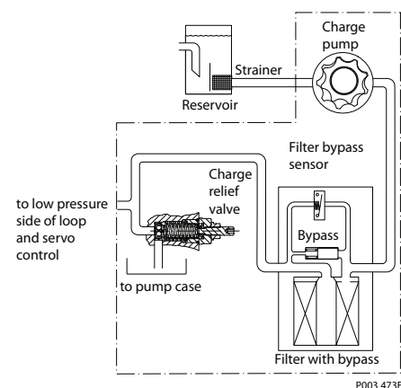
Integral charge pressure filtration, full flow
