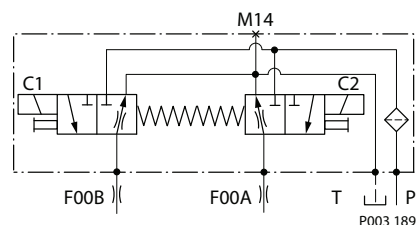
3-Position electric control, hydraulic schematic
