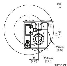
Remote charge pressure filtration, full flow
