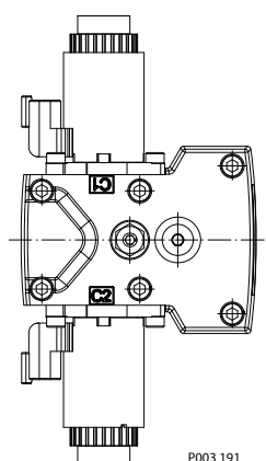
EDC control
