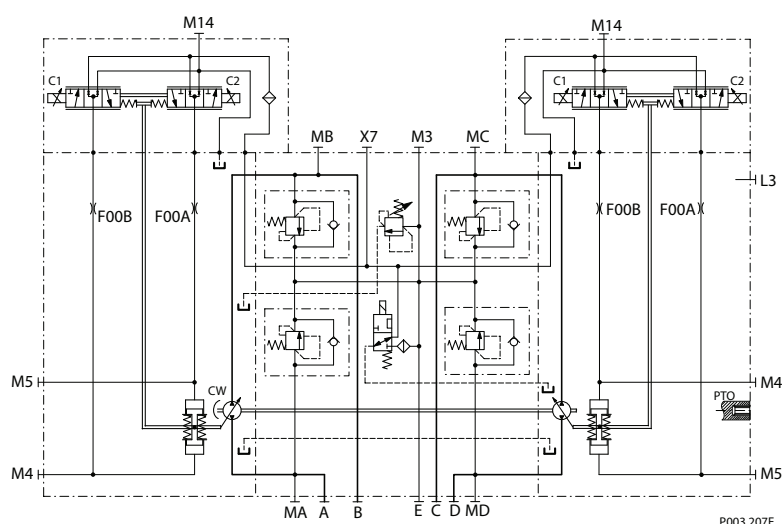
System schematic, tandem pump
