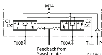
EDC schematic
