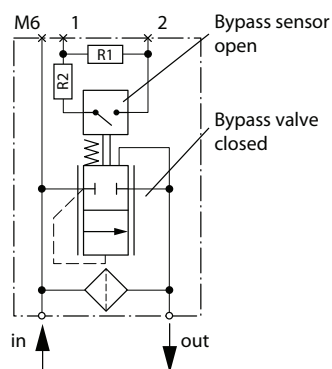
Schematic
