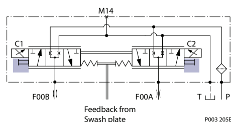
MOR-Schematic diagram (EDC shown)
