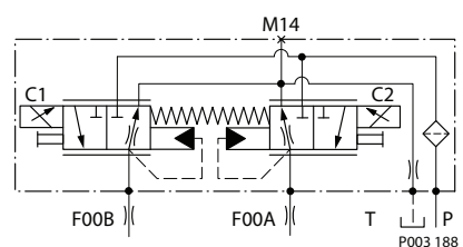
NFPE schematic
