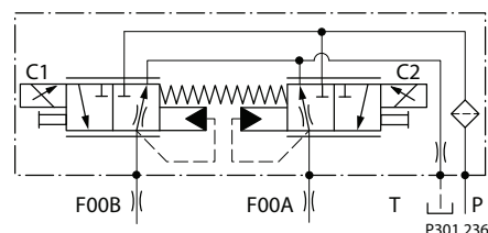
Automotive Control (AC) schematic
