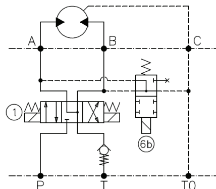
Figure 31. Freewheeling circuit with a 4/2 valve.
