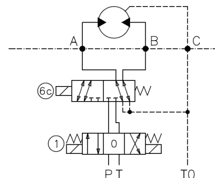
Figure 32. Freewheeling circuit with a 6/2 valve.
