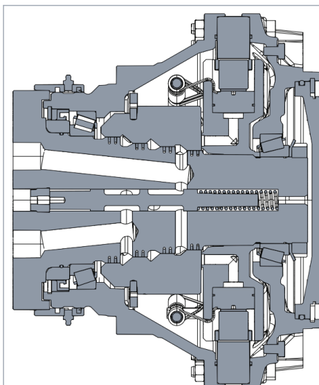
Figure 18. 2-speed motor.
