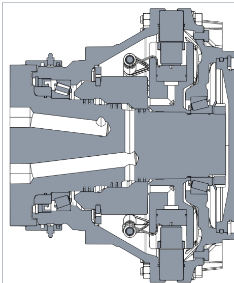
Figure 16. 1-speed motor.
