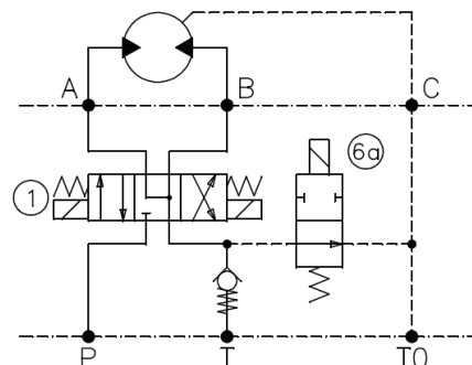
Figure 30. Freewheeling circuit with a 2/2 valve.
