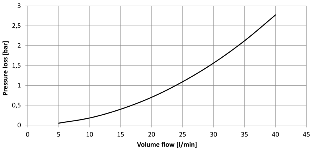
Picture 1 Pressure loss vs coolant flow
