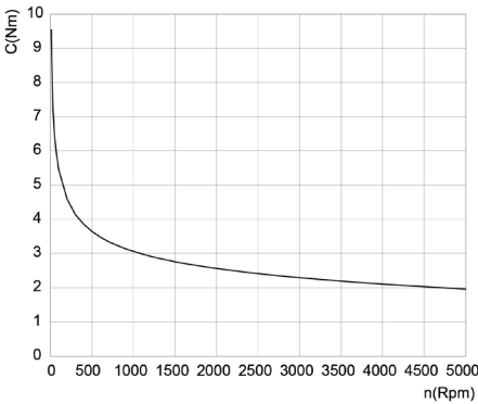
PM-6E 40... C = Torque [Nm] n = number of revolutions per minute [Rpm]
