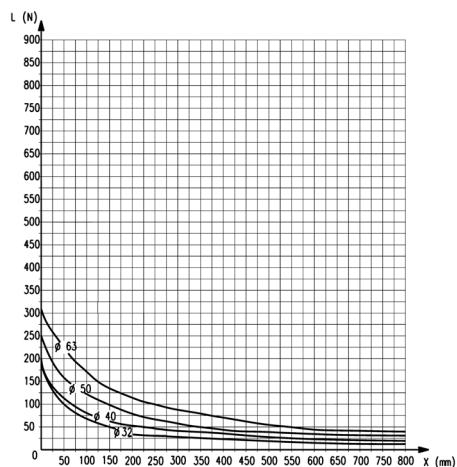
Guide "U" moving on bush (45NUT)
