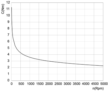
PM-6E 63... C = Torque [Nm] n = number of revolutions per minute [Rpm]
