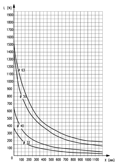
Guide "HT" moving on bush (45NHT)
