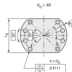
Drilling pattern 2
