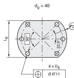
Drilling pattern 1
