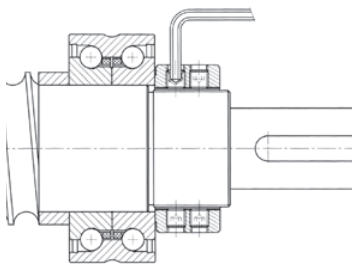
LRP nuts for mounting and set up of a ball screw.
