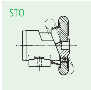
Foot mounted without shaft end
