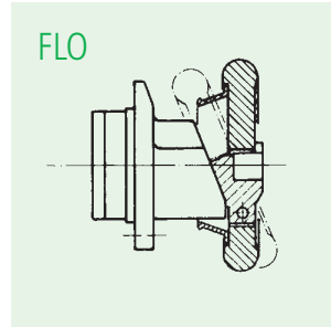
Flange mounted without shaft end
