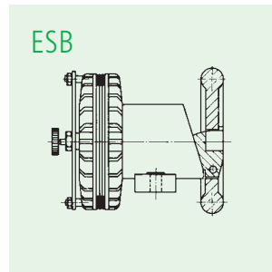
Single disk brake
