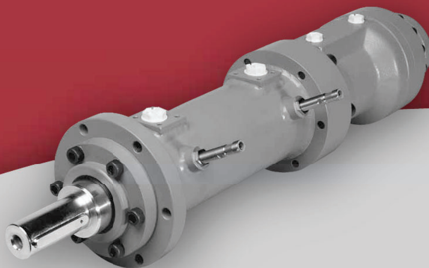
Rotary-linear actuator HSE4 Hydraulic / 100 bar
