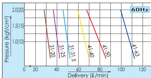
Pump/Motor Combination
