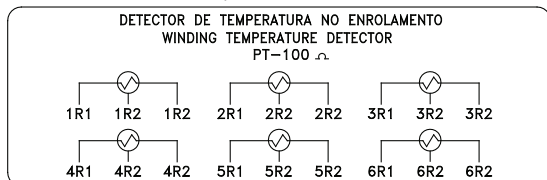
Figure 29 - Additional nameplate for winding temperature detectors (Pt-100).
