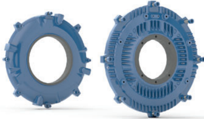
Figure 20 - DE endshield (left) and NDE endshield (right).
