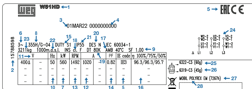
Figure 28 - Main nameplate of the motor.
