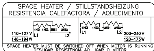
Figure 31 - Additional nameplate for the space heater.
