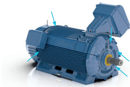
Figure 39 - Location of vibration measuring points.
