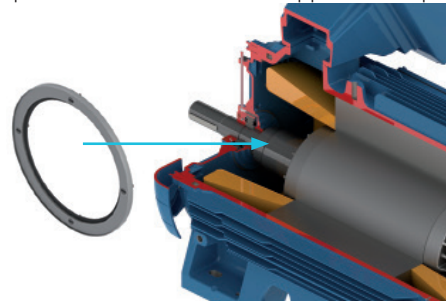
Figure 13 - AEGIS grounding ring.
