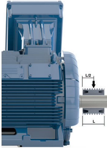
Figure 46 - Radial load applied to the shaft end.
