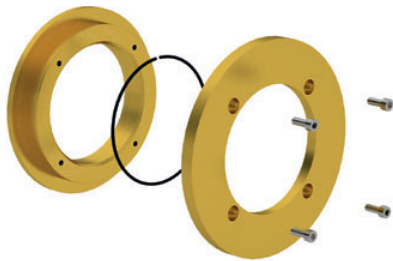
Figure 48 - Taconite Labyrinth
