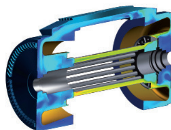
Figure 33 - Demonstration of the airflow through the rotor holes.
