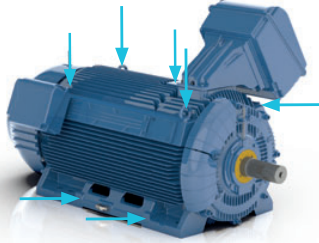
Figure 3 - Eyebolt fixing points for motors with feet.
