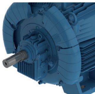
Figure 26 - Two pairs of air baffles for motors with sleeve bearings.
