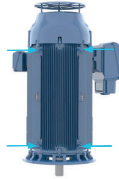
Figure 6 - Eyebolt fixing points for lifting footless motors (at the top side).
