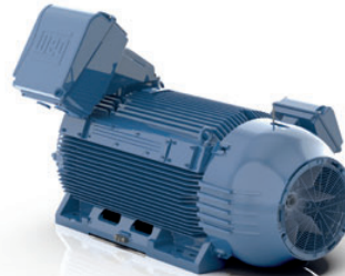
Figure 23 - Fan cover manufactured in cast iron FC-200.
