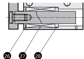
Ball bearing
