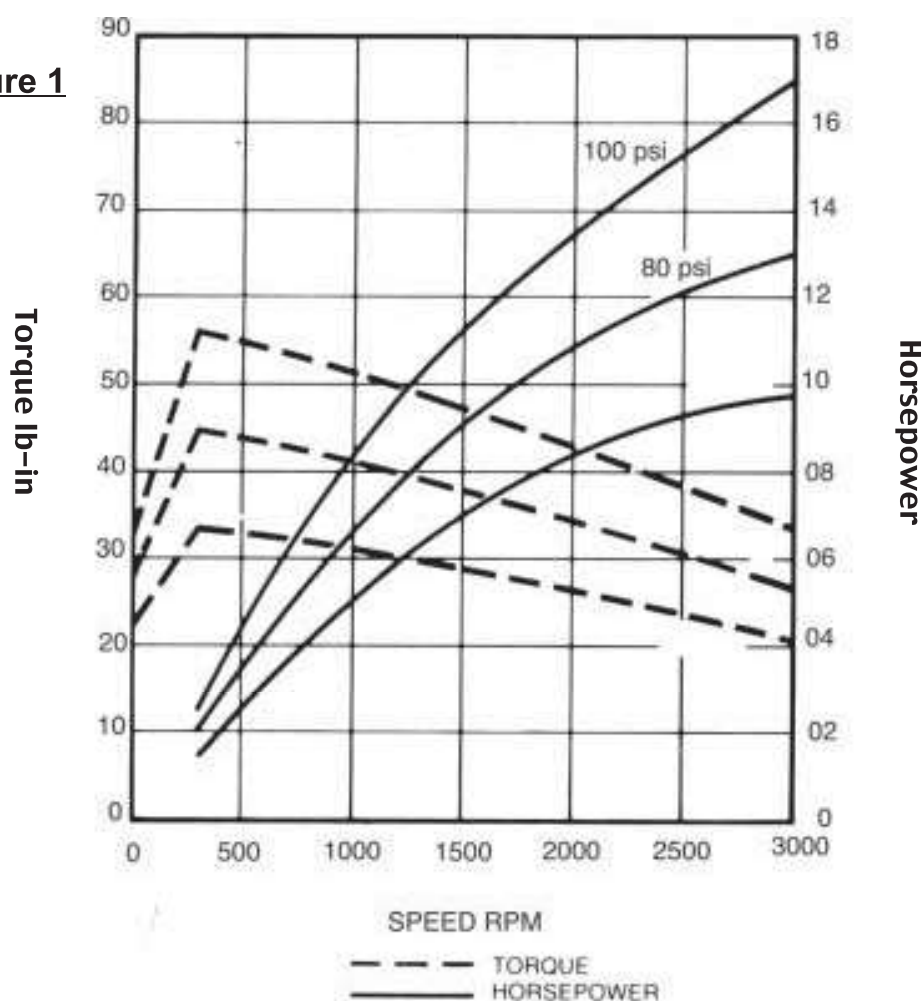
Horsepower-torque characteristics of typical rotary vane air motor
