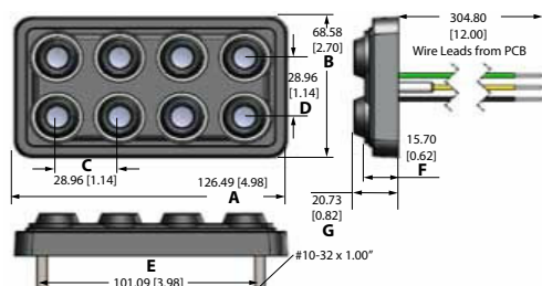
HMK-24 dimensions in mm [in]
