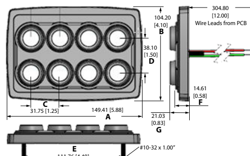
HMK-24L dimensions in mm [in]
