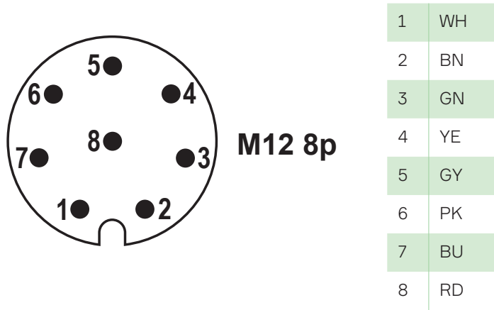
Figure 5 M12 8p
