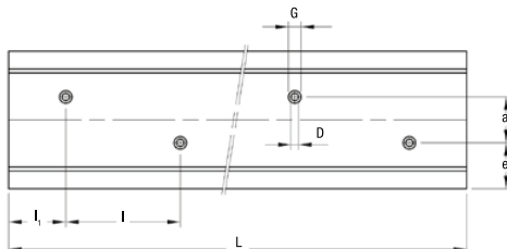
Hole layout for LM 90, LM 120
