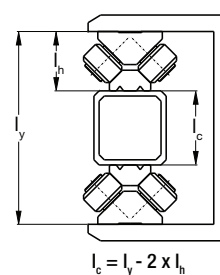
Guide between the rollers
