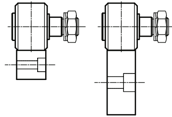
LAYOUT 1 HOLE PATTERN A AND B
