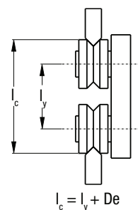
Guides outside the rollers
