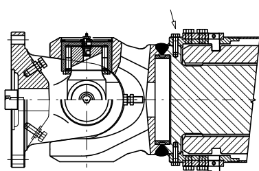
SHEAR PIN SAFETY DEVICE
