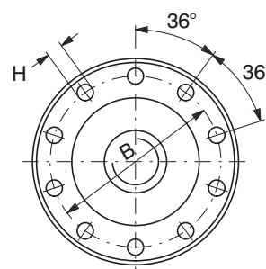
SIZE 31 - 39 10 HOLES
