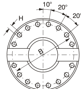
SIZE 39 - 62 16 HOLES
