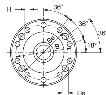
SIZE 31 - 39 10 HOLES
