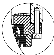
SIZES 44 ÷ 62
