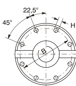
SIZE 18 - 25 8 HOLES
