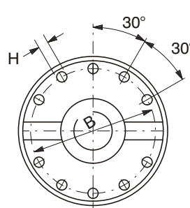
SIZE 28 - 35 10 HOLES
