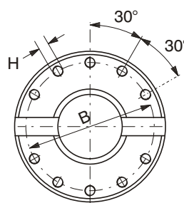
SIZE 31 - 39 10 HOLES
