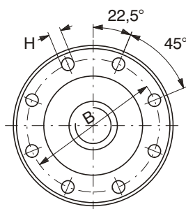
SIZE 18 - 28 8 HOLES
