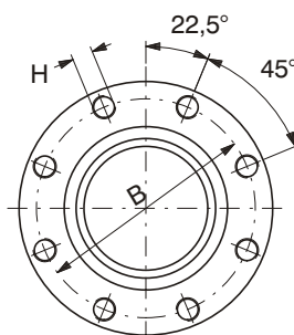
SIZE 18 - 28 8 HOLES
