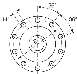
SIZE 31 - 39 10 HOLES
