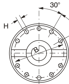
SIZE 31 - 39 10 HOLES
