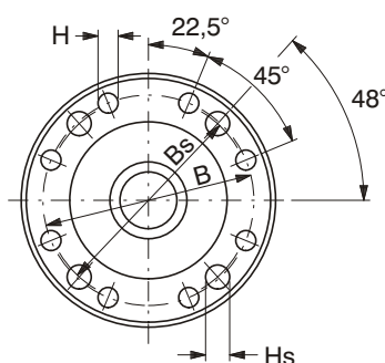
SIZE 18 - 28 8 HOLES
