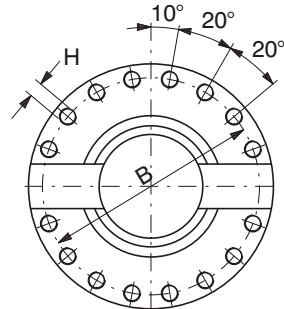
SIZE 39 - 62 16 HOLES
