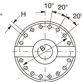
SIZE 44 - 62 16 HOLES
