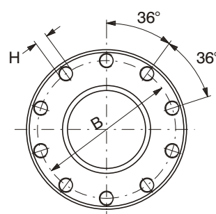
SIZE 31 - 39 10 HOLES
