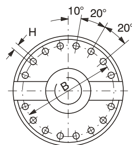
SIZE 39 - 62 16 HOLES
