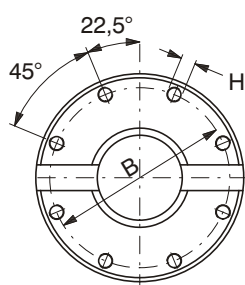
SIZE 18 - 28 8 HOLES
