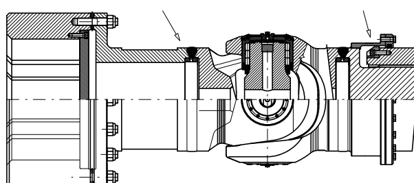
QUICK ENGAGEMENT
