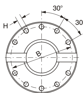
SIZE 28 - 35 10 HOLES
