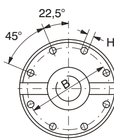
SIZE 18 - 28 8 HOLES
