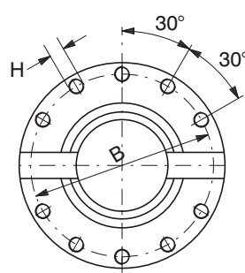
SIZE 28 - 35 10 HOLES
