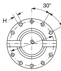
SIZE 31 - 39 10 HOLES
