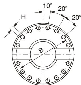
SIZE 44 - 62 16 HOLES
