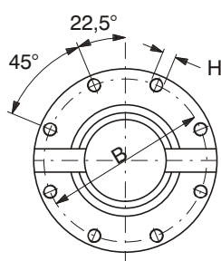
SIZE 18 - 28 8 HOLES
