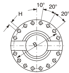
SIZE 44 - 62 16 HOLES
