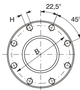
SIZE 18 - 28 8 HOLES
