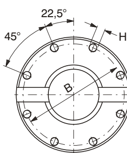
SIZE 18 - 25 8 HOLES
