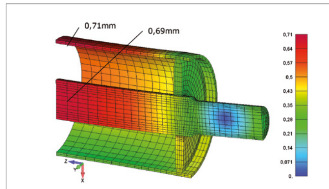
Deformation on an belt drum
